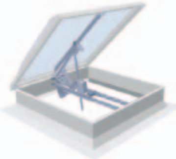
Flügelstrebe, Adapterbleche und Montagematerial / sash rod, adapter plates and mounting material
